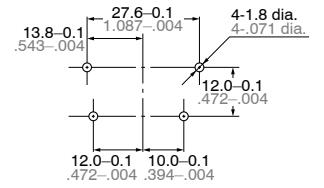
(Copper-side view)
