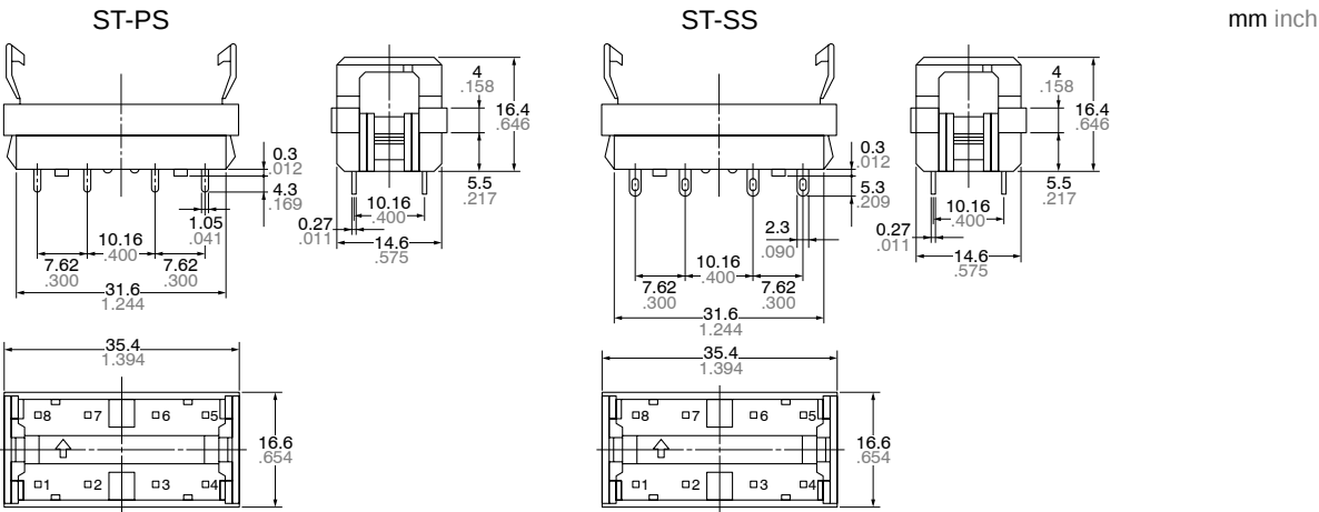
ST-PS PC board terminal socket
