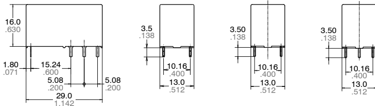
Single side stable type 1 coil latching type 2 coil latching type
