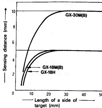
• Target size - Sensing distance correlation
