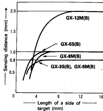
• Target size - Sensing distance correlation
