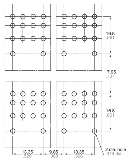
Side-by-side installation
