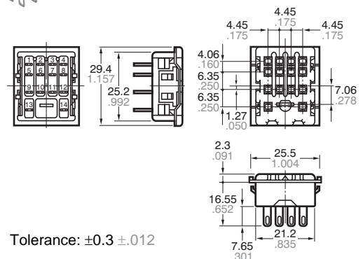
External dimensions
