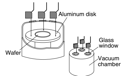
Inner-chamber evenness detection
