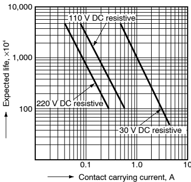
1.-(1) Life curve (DC load 2 Form C, 4 Form C)
