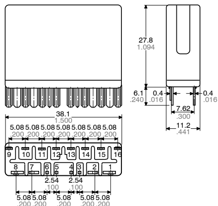
External dimensions
