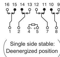
Schematic (Top view)
